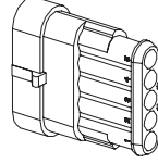
Housing SR CODE 8032212 SEAL 8032209
